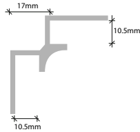
Type V Internal Corner
